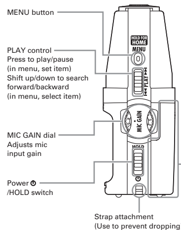
Right side
