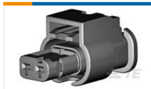
TE Part #1-1670916-1 2POS, MCON 1.2 LL REC SEALED
