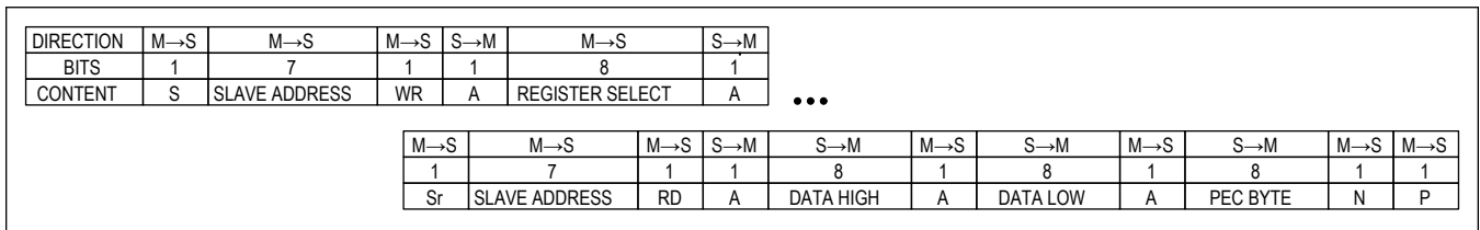
Figure 5. 2-Byte Read from MAX31827 with PEC Byte.
