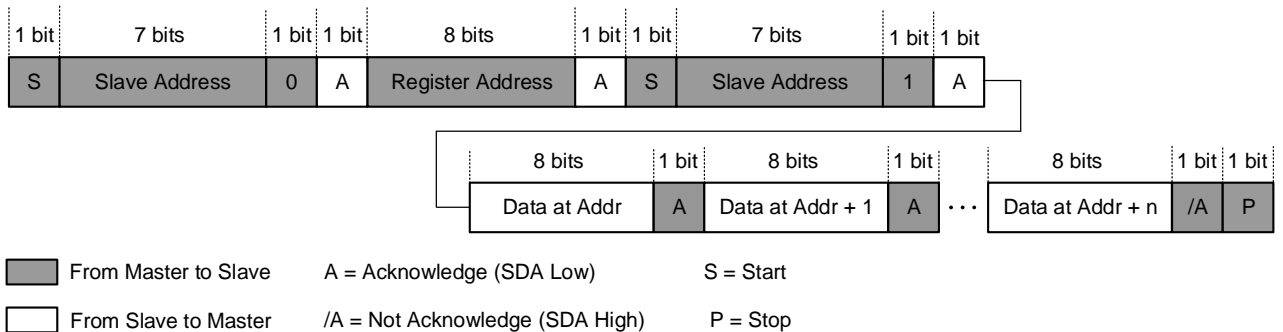
Figure 17: Multi-Read
