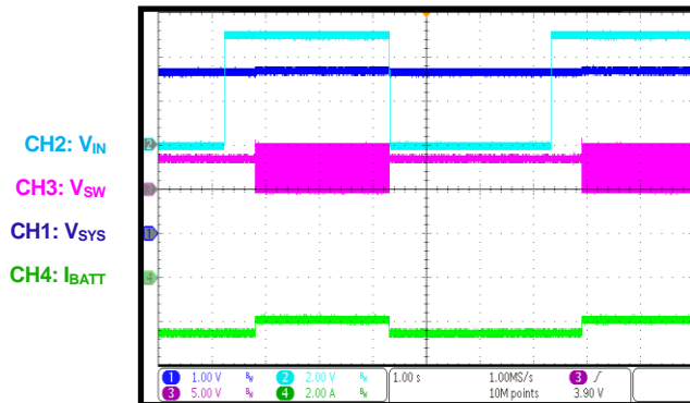
Power-On/Off Waveform V IN = 5V, I IN_LIM = 500mA, V BATT = 3.8V, I sys = 2.5A
