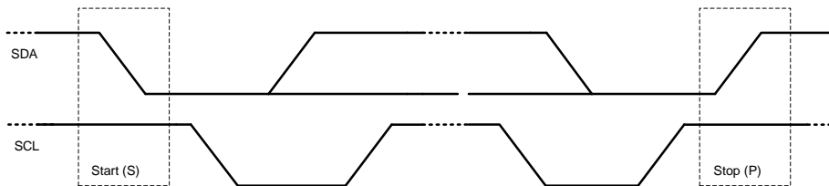
Figure 11: Start and Stop Conditions
