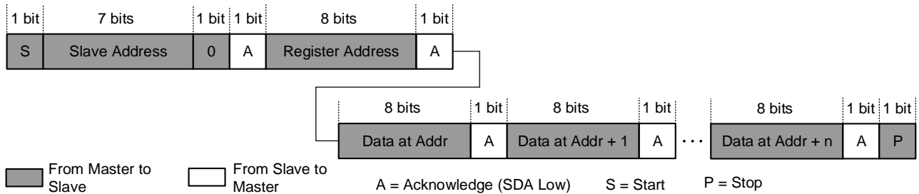
Figure 16: Multi-Write
