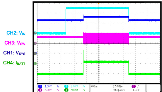
Power-On/Off Waveform V IN = 5V, I IN_LIM = 500mA, V BATT = 3.3V, I sys = 0.5A
