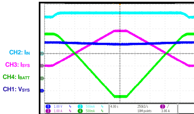
Input Current Limit V IN = 5V, V BATT = 3.8V, I IN_LIM = 1800mA
