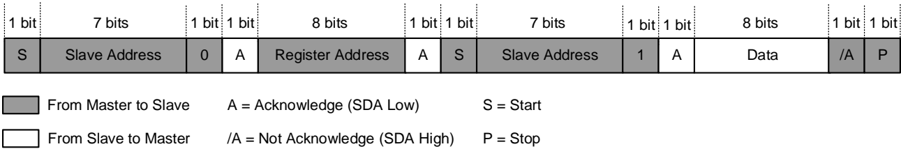
Figure 15: Single Read
