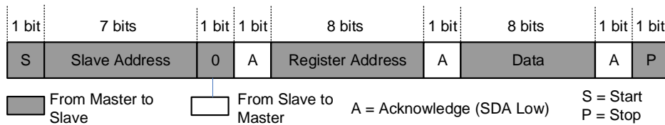
Figure 14: Single Write
