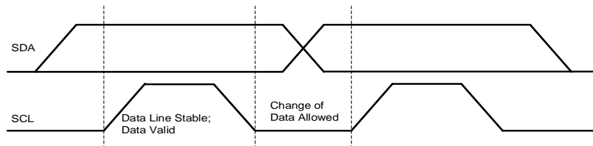
Figure 10: Bit Transfer on the I 2 C Bus
