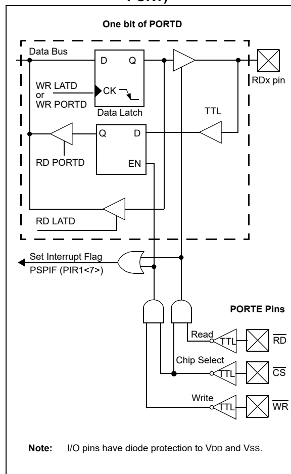
FIGURE 10-2: PORTD AND PORTE BLOCK DIAGRAM (PARALLEL CLIENT PORT)
