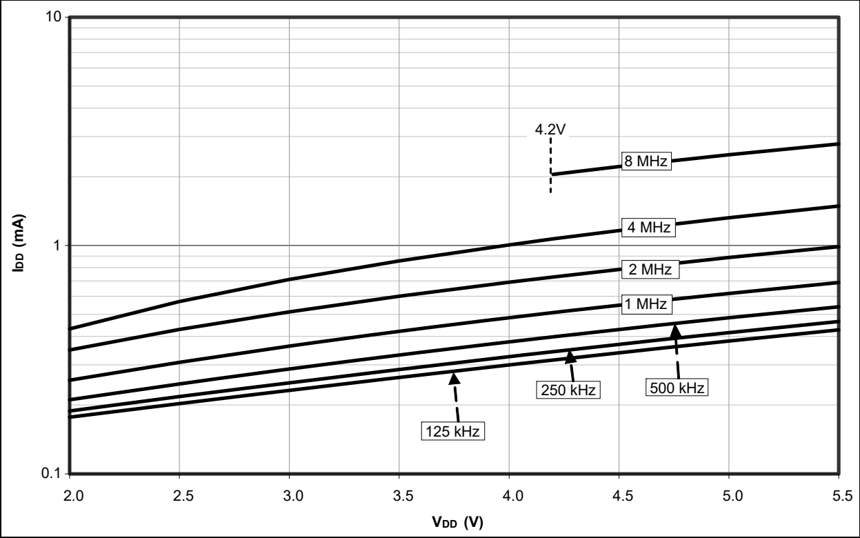
FIGURE 27-15: MAXIMUM I_{DD} ACROSS V_{DD} (RC_IDLE MODE, -40°C TO +85°C)
