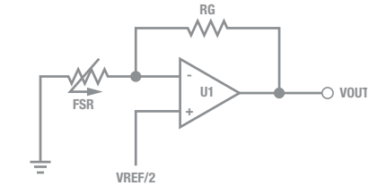
Figure 9. Alternative force sensor current to voltage converter.
