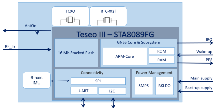
Figure 1. Block schematic
