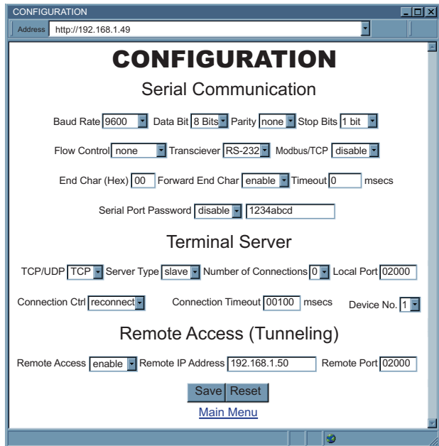
Figure 4.16 Local iServer (Serial-to-Ethernet model) Configuration Page
