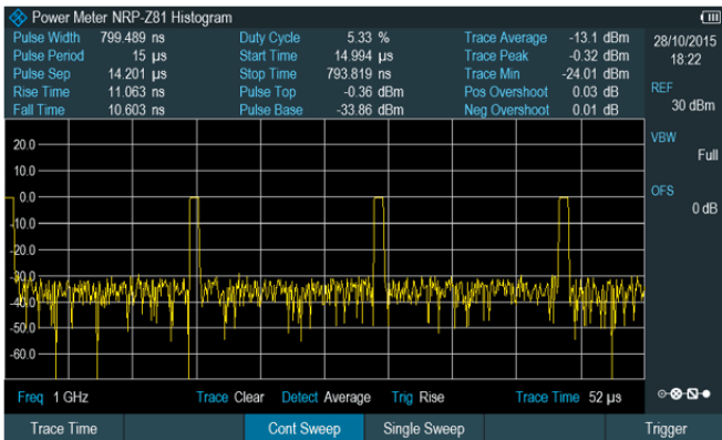
Pulse analysis with R&S®ZNH-K29 and R&S®NRP-Z81 wideband power sensors.
