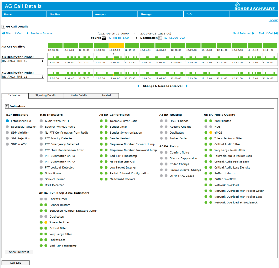
R&S®AVQA air-ground monitor indicates the exact timing and root cause of an impairment.
