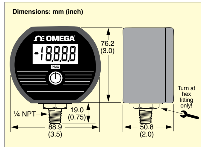
DPG3500 Dimensions
