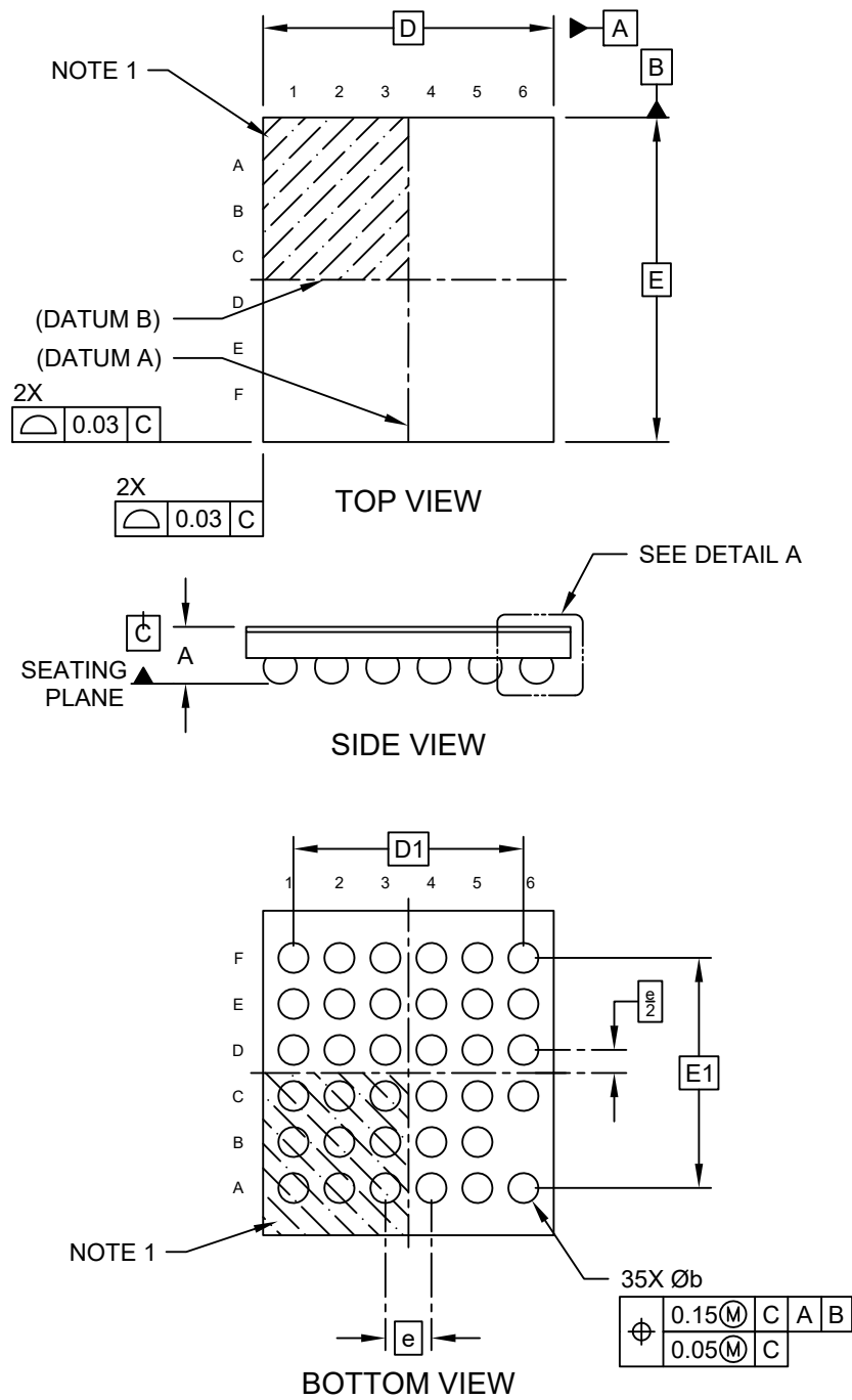
Microchip Technology Drawing C04-21245 Rev A Sheet 1 of 2
