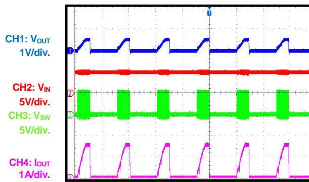
Short-Circuit Steady
