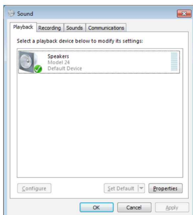
Windows 7 screen
