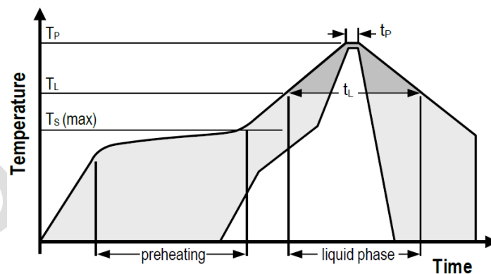
Figure 19 Soldering profile according to JEDEC standard. Recommended conditions are T_P = 245^\circ\text{C} and t_P \leq 30\text{ s} for Pb-free assembly, T_L < 220^\circ\text{C} and t_L < 150\text{ s} . Ramp-up rate <3^\circ\text{C s}^{-1} and ramp-down rate <4^\circ\text{C s}^{-1} .
