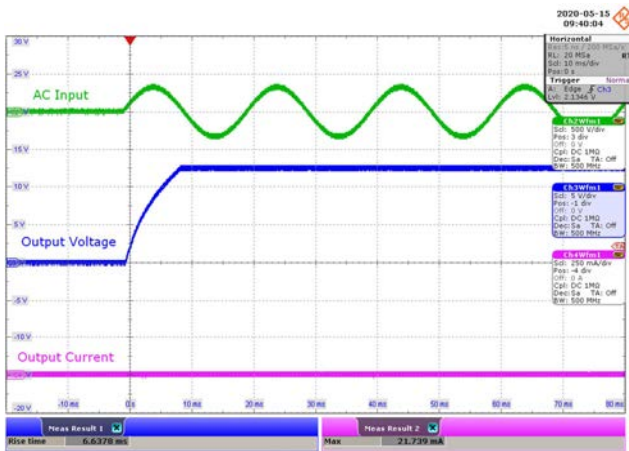
Figure 65 – 230 VAC 50 Hz.
