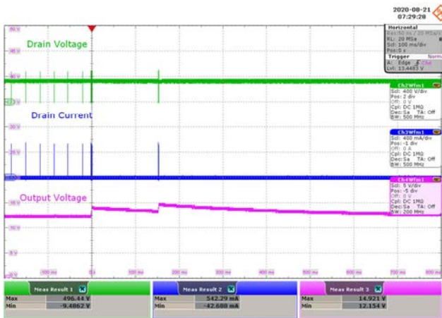
Figure 109 – 230 VAC 50 Hz.
