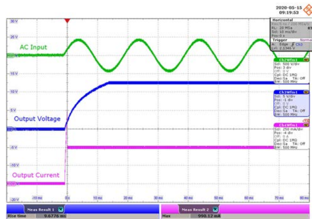
Figure 54 – 300 VAC 50 Hz.
