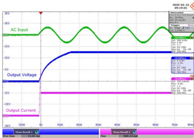
Figure 53 – 230 VAC 50 Hz.
