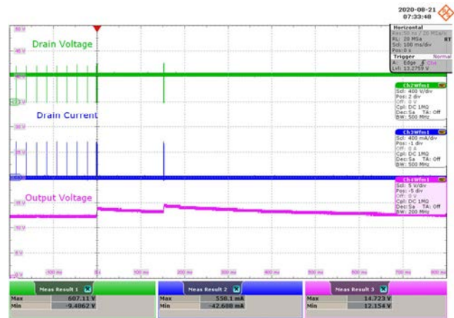
Figure 110 – 300 VAC 50 Hz.
