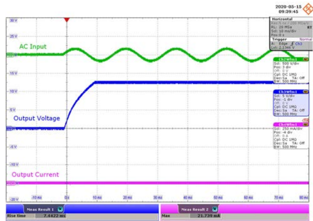
Figure 64 – 115 VAC 60 Hz.
