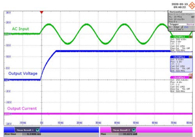
Figure 66 – 265 VAC 50 Hz.
