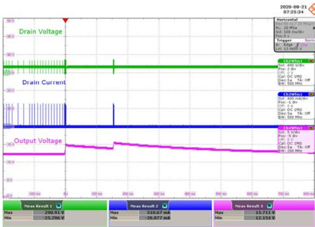
Figure 107 – 90 VAC 60 Hz.
