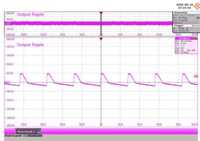
Figure 118 – 300 VAC 50 Hz.
