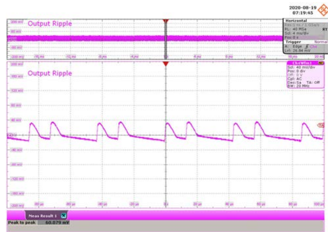
Figure 116 – 115 VAC 60 Hz.
