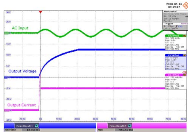
Figure 52 – 115 VAC 60 Hz.
