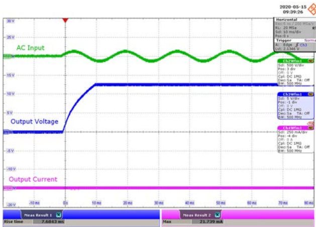
Figure 63 – 90 VAC 60 Hz.
