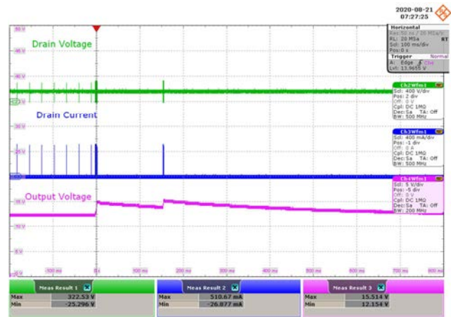
Figure 108 – 115 VAC 60 Hz.
