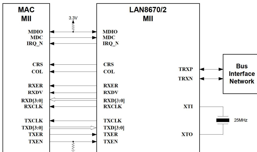
Figure 6-1. MII Connectivity
