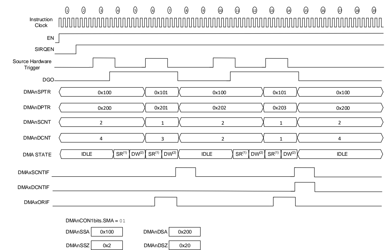
Figure 16-10. Overrun Interrupt
