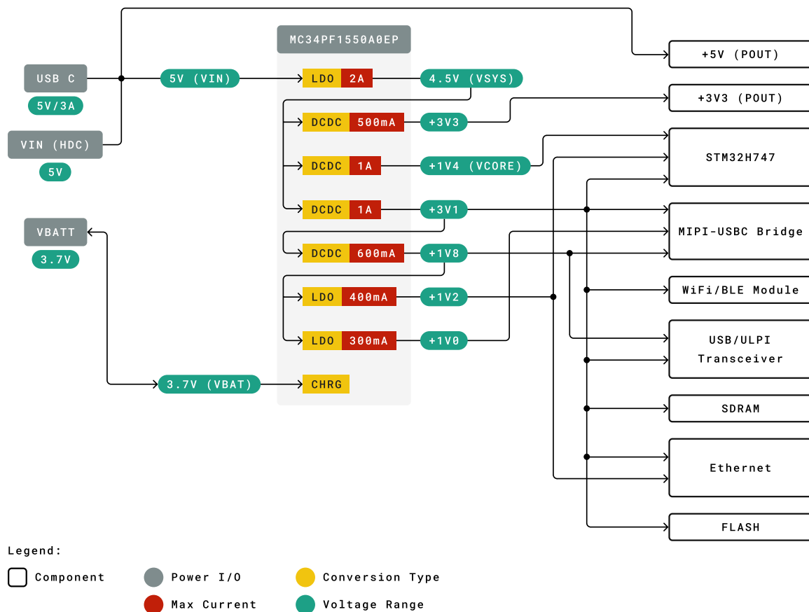
Portenta H7 Lite Connected Power Tree
