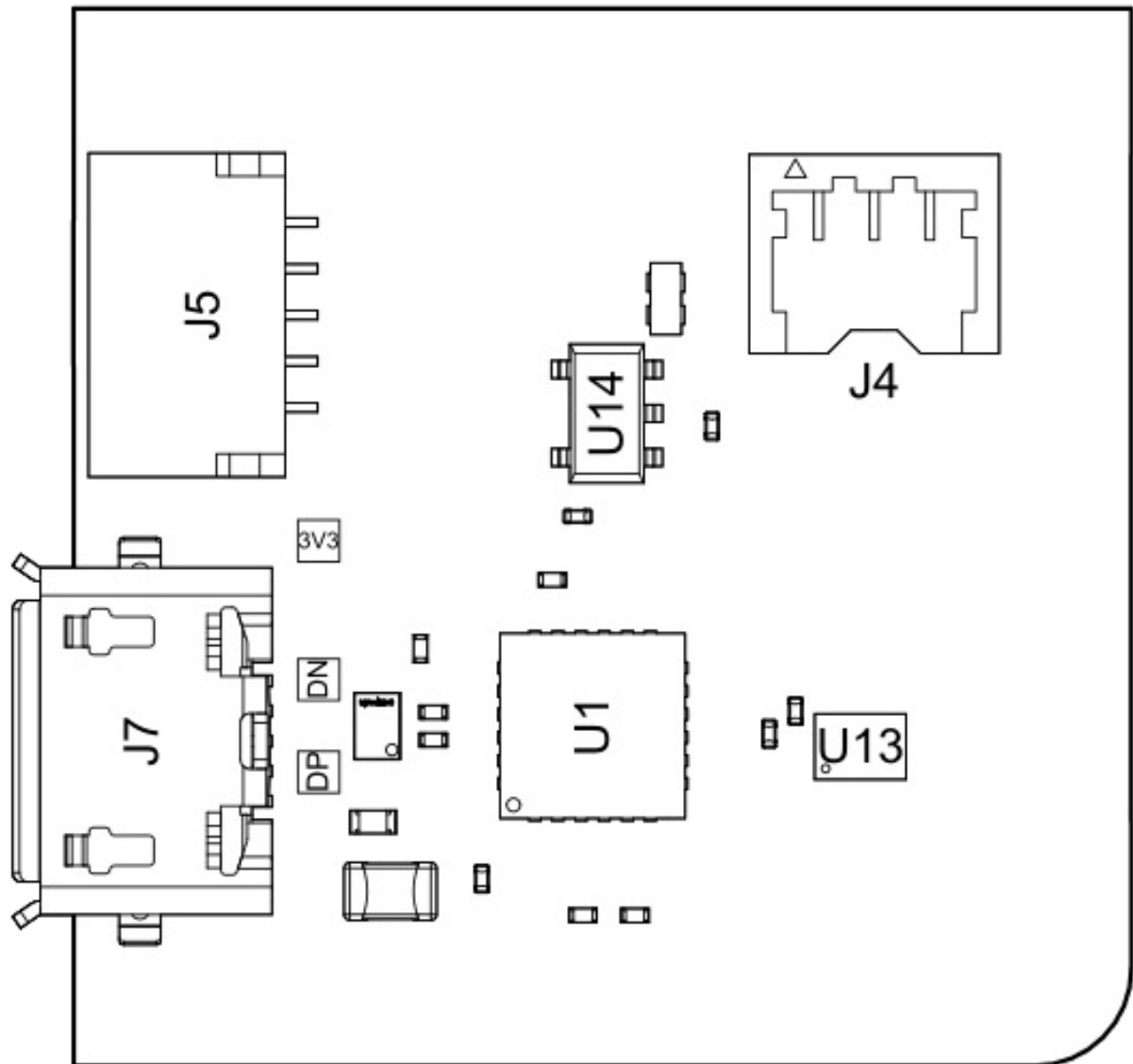
Nicla Sense ME Back View
