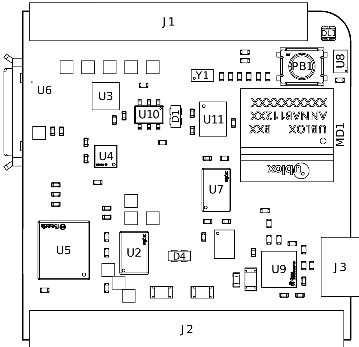
Nicla Sense ME Top View
