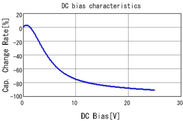
GRM188R61E225KA12 C-DC bias capchange, 25.0degC, A
