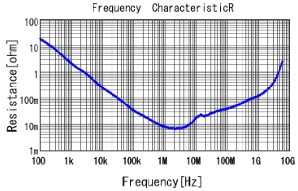
GRM188R61E225KA12 R DCOV, 25degC
