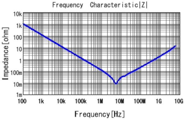
GRM188R61E225KA12 |Z| DCOV, 25degC
