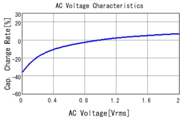
GRM188R61E225KA12 C-AC Voltage capchange, DCOV, 25
