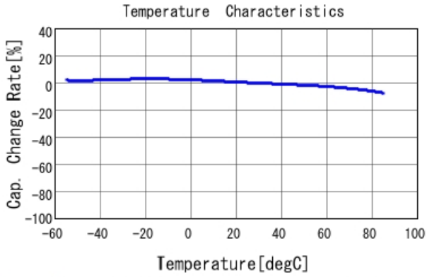
GRM188R61E225KA12 C-Temp. capchange, DC0.0V, AC1.C
