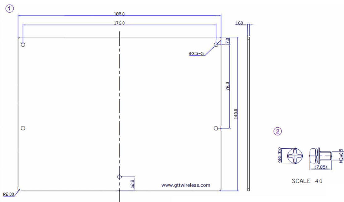
Adaptor Board for GLB Enclosure
