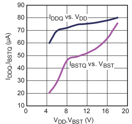
Quiescent Current vs. Voltage
