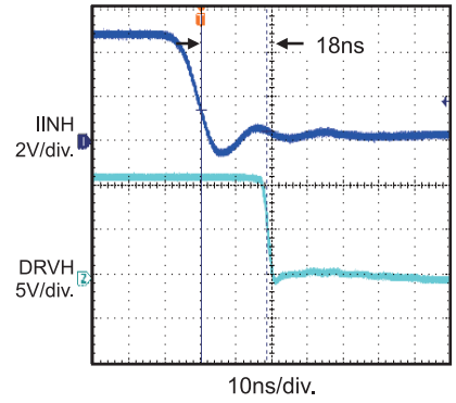
Turn-off Protection Delay
