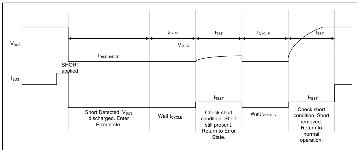
FIGURE 6-6: Error Recovery.
