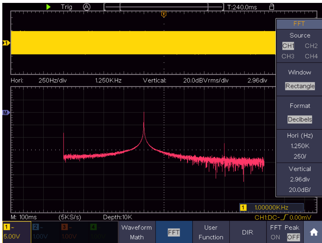
Figure 4-2 Rectangle window
