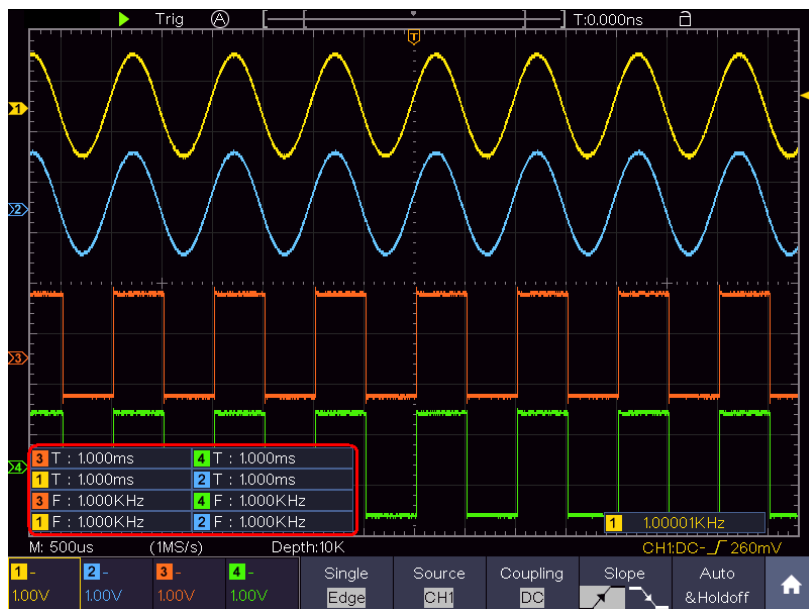
Figure 4-24 Automatic measurement
