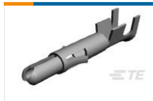
TE Part #350705-1 UMNL SPLIT PIN 20-14 PTPBR L/P
