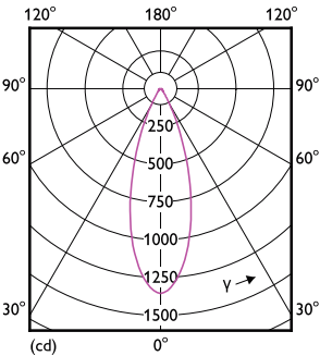
LEDspots MAS IC 7,5W MR16 GU5,3 930 36D-LDD
