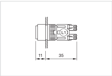
Dimensions [mm] L1 = Solder terminal 2.8 x 0.5 mm
