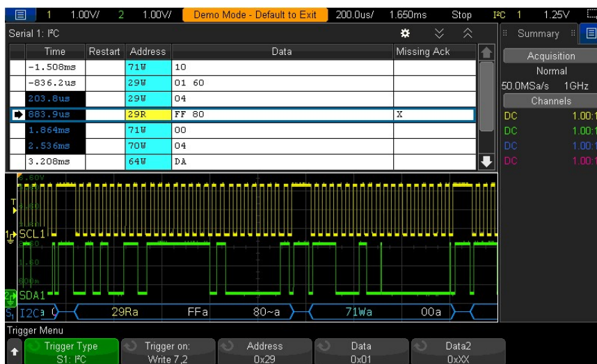
Figure 16. I 2 C decode and trigger.
