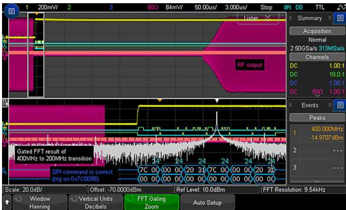
Figure 21. Triggered on a SPI command, the RF signal is still at 400 MHz as indicated in the frequency peak search result list.
