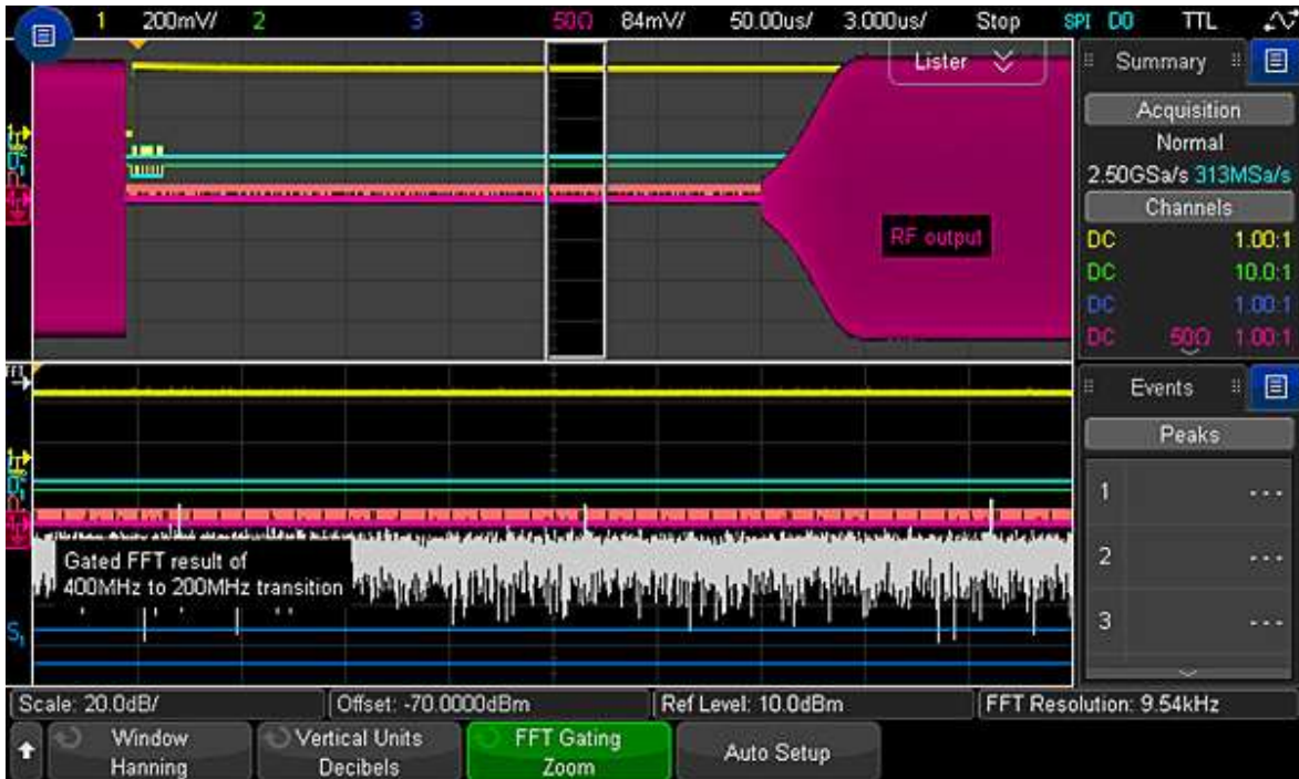
Figure 22. No RF activities in this zoomed time.
