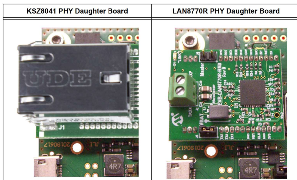
FIGURE 2-1: LAN PHY DAUGHTER BOARD EXAMPLES
