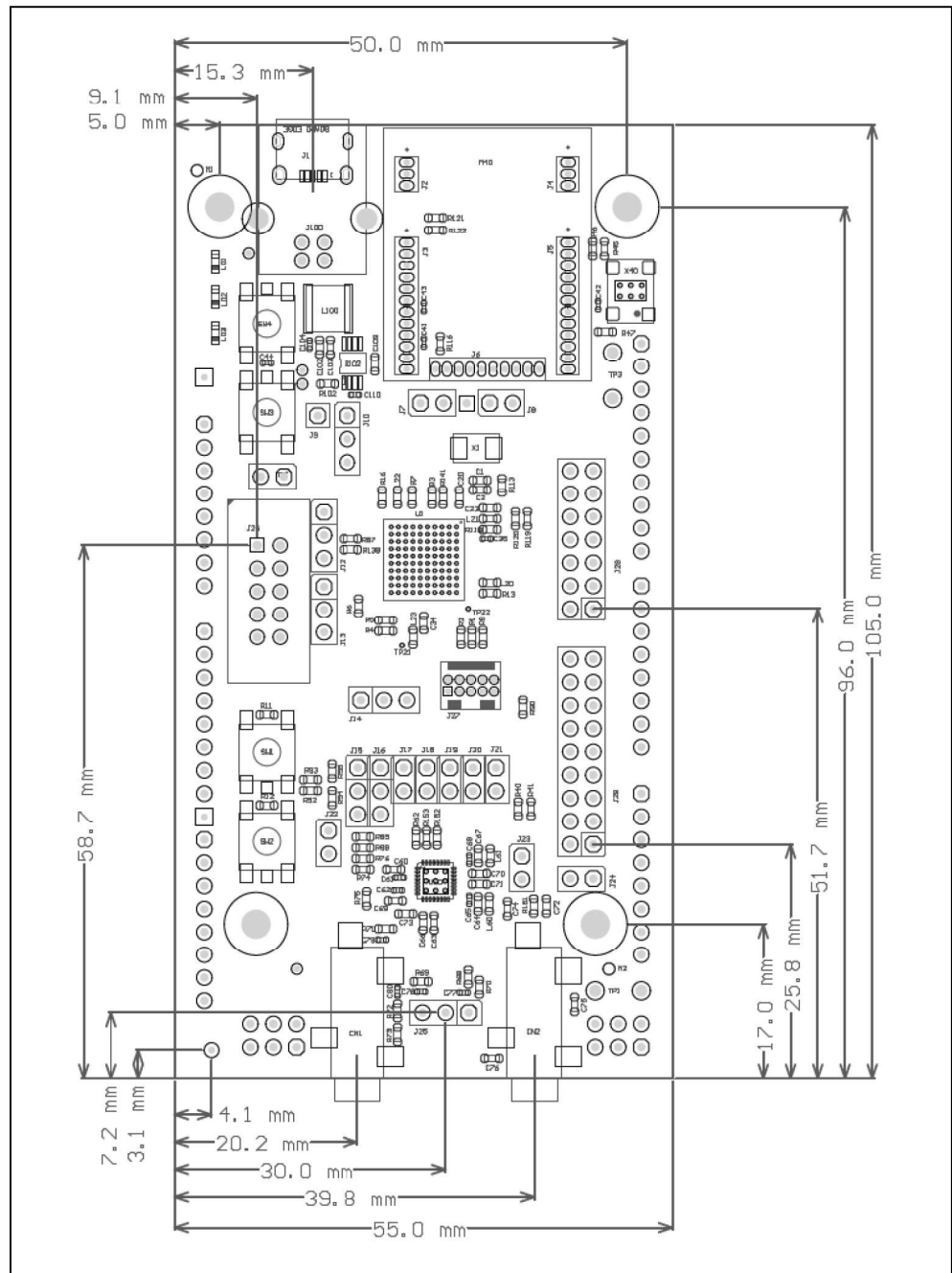
FIGURE 5-1: ASSEMBLY PLAN – TOP VIEW AND MECHANICAL DIMENSIONS
