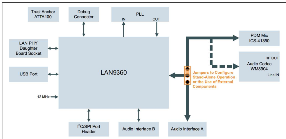
FIGURE 1-2: BLOCK DIAGRAM
