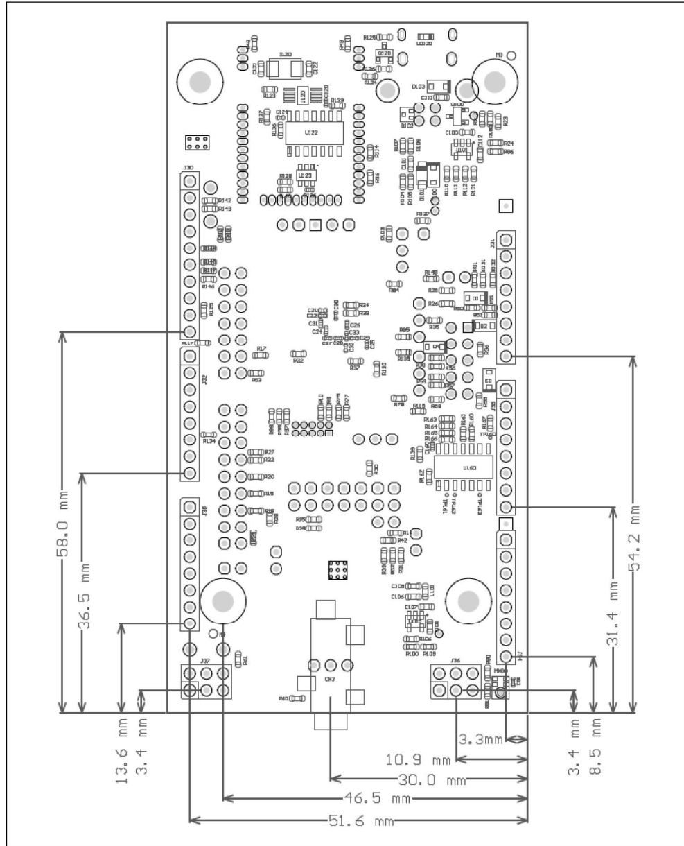
FIGURE 5-2: ASSEMBLY PLAN – BOTTOM VIEW AND MECHANICAL DIMENSIONS
