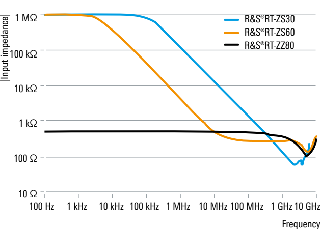
Input impedance versus frequency
