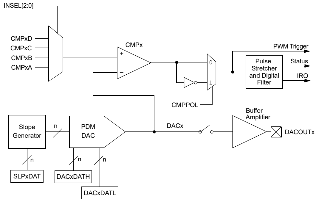
Figure 14-1. High-Speed Analog Comparator Module Block Diagram
