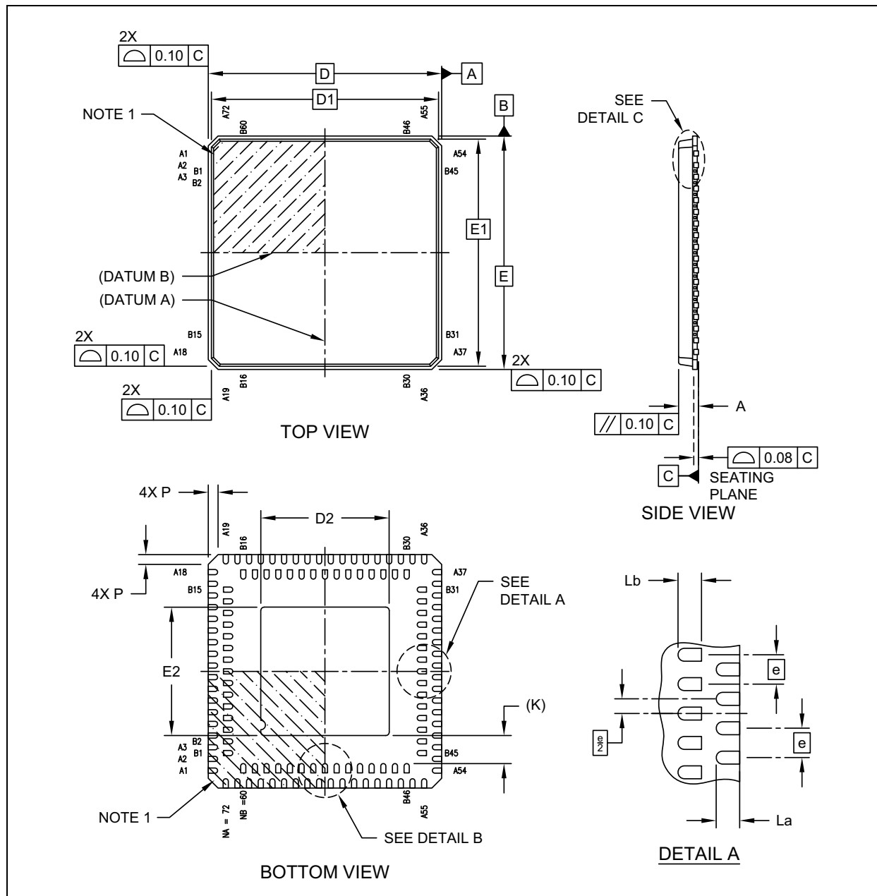
FIGURE 42-2: PIC32MZ1025W104 SOC PACKAGE DRAWINGS
