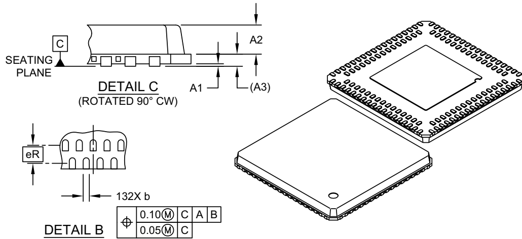
FIGURE 42-3: PIC32MZ1025W104 SOC PACKAGE DRAWINGS – CONTD.,
