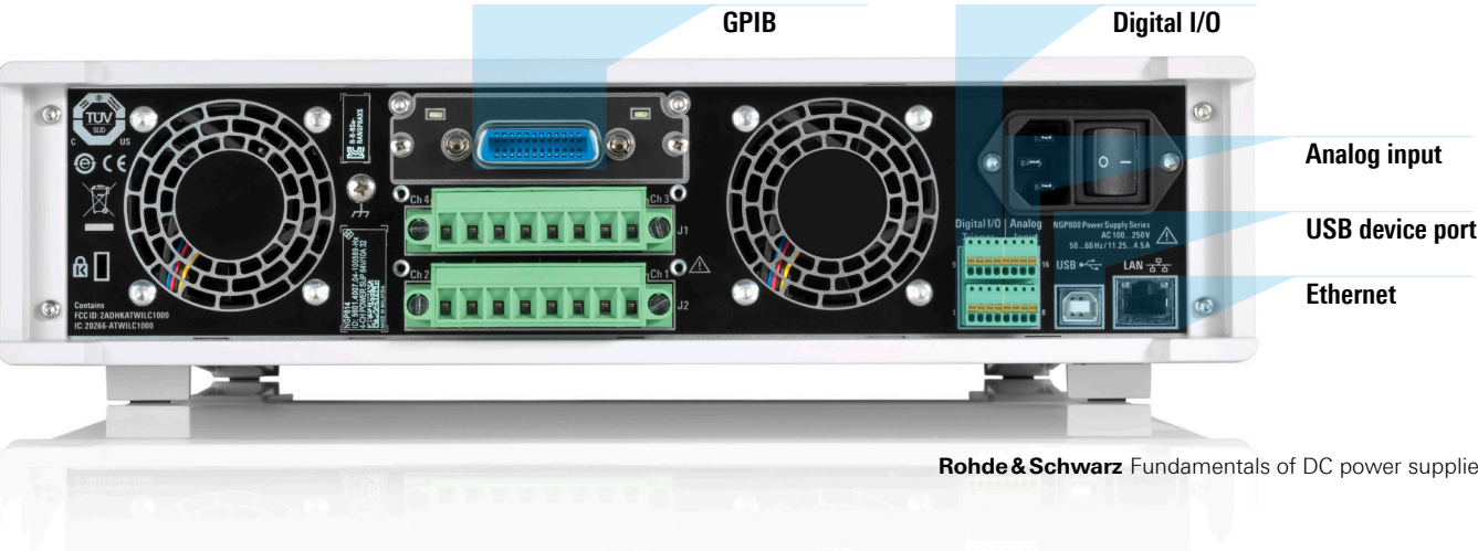
Rear view of an R&S®NGP800 power supply with interface ports
