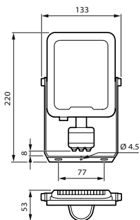
BVP164 LED36/840 PSU 30W SWB MDU CE
