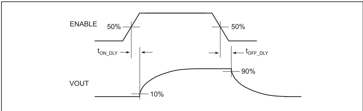
FIGURE 1-2: Switching Delay Times.
