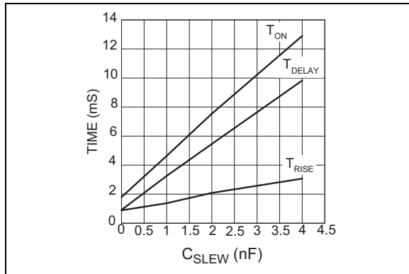
FIGURE 5-5: C_{SLEW} vs. Turn-On, Delay and Rise Times.
