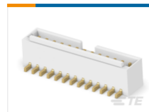
TE Part # 3-2380320-3 1.5P 13POS WTB VERT BRD W LATCH AU NAT
