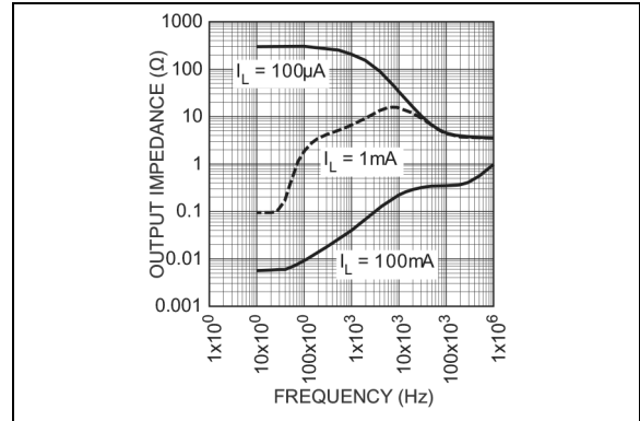
FIGURE 2-22: Output Impedance.
