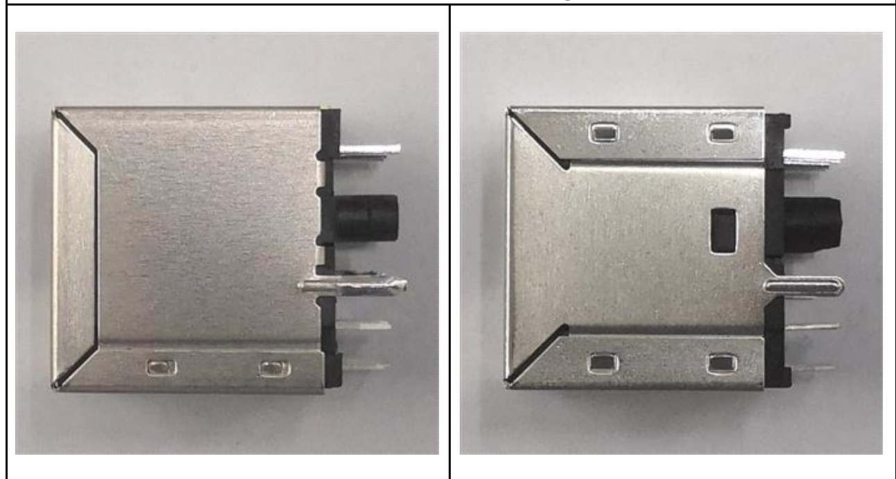
Above: The RJ45 shield will be closed on both sides while assembly to make the assembly easier.
