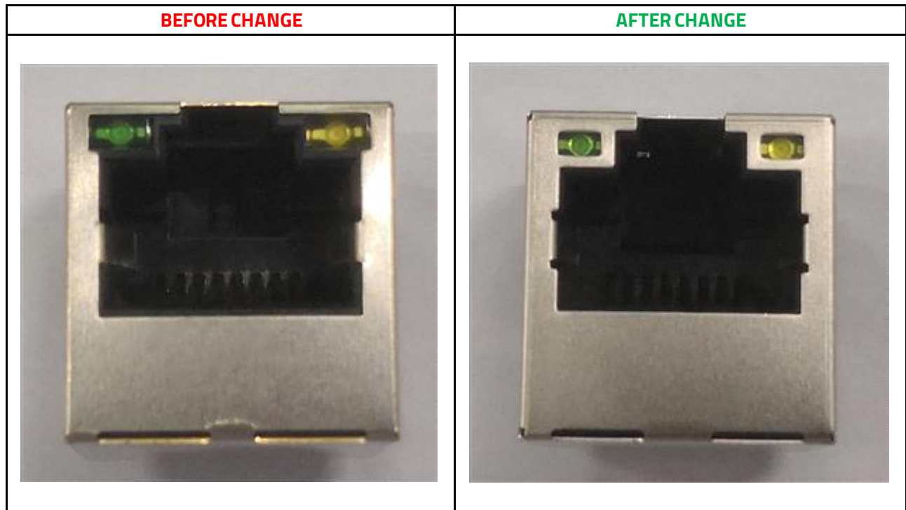
Above: The shield of the RJ45 is covering the LEDs.
