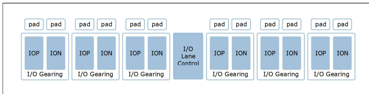
Figure 6-3. I/O Topology
