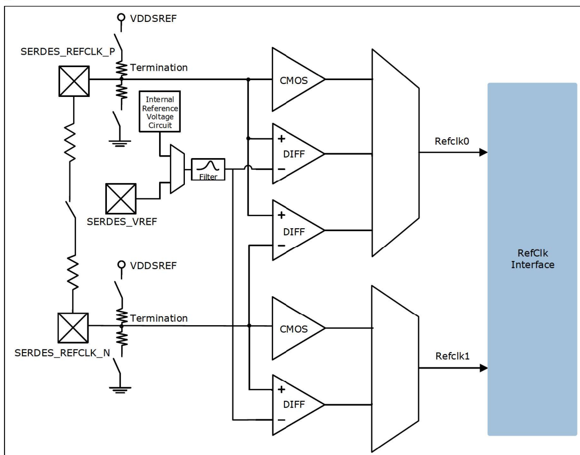
Figure 6-2. Reference Clock
