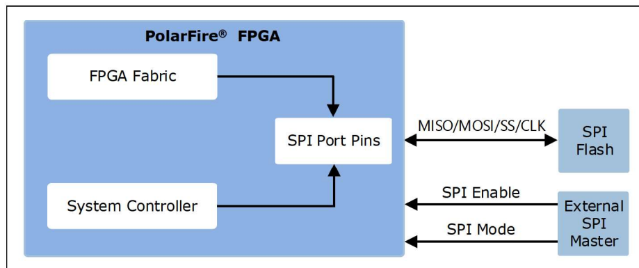
Figure 10-1. SPI Programming Port
