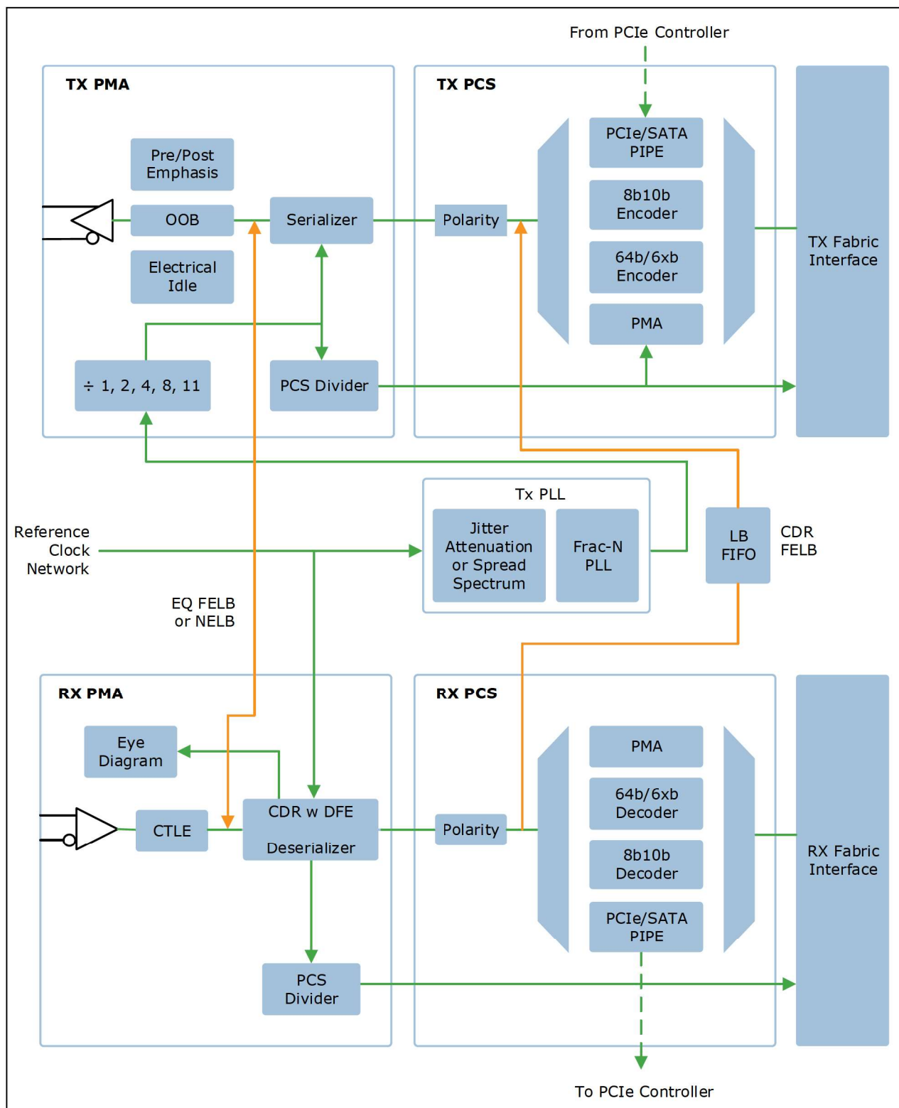
Figure 6-1. Transceiver Lane Modes
