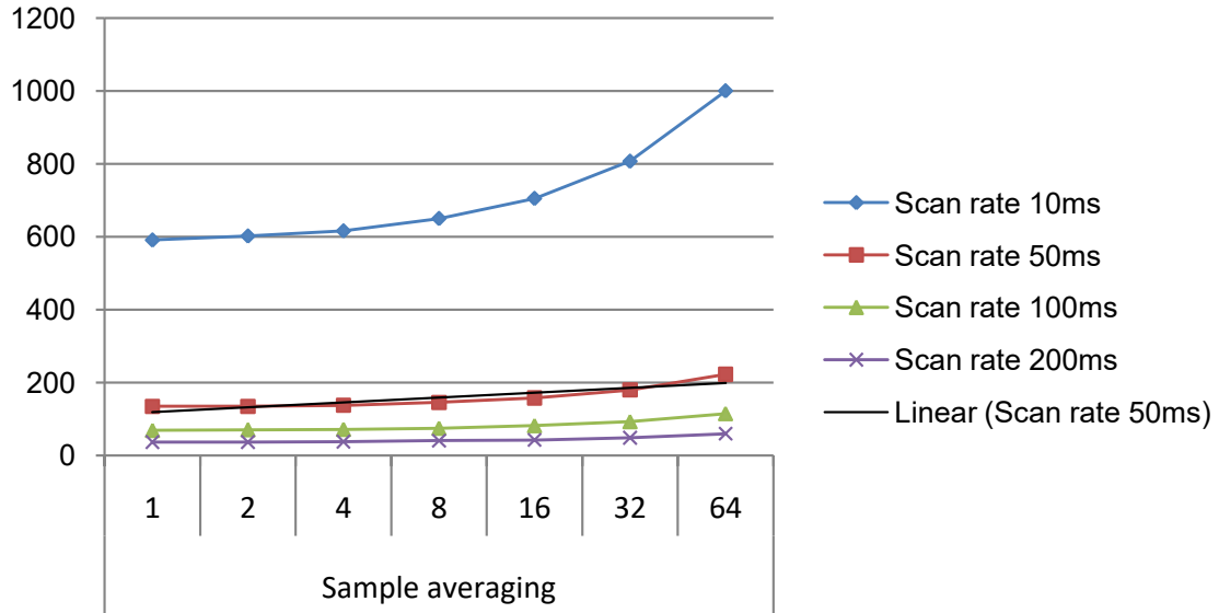
Figure 32-10. Power Consumption [ \mu A] 10 sensors, noise countermeasures Enabled, f=48\text{MHz} , V_{CC}=3.3\text{V}
