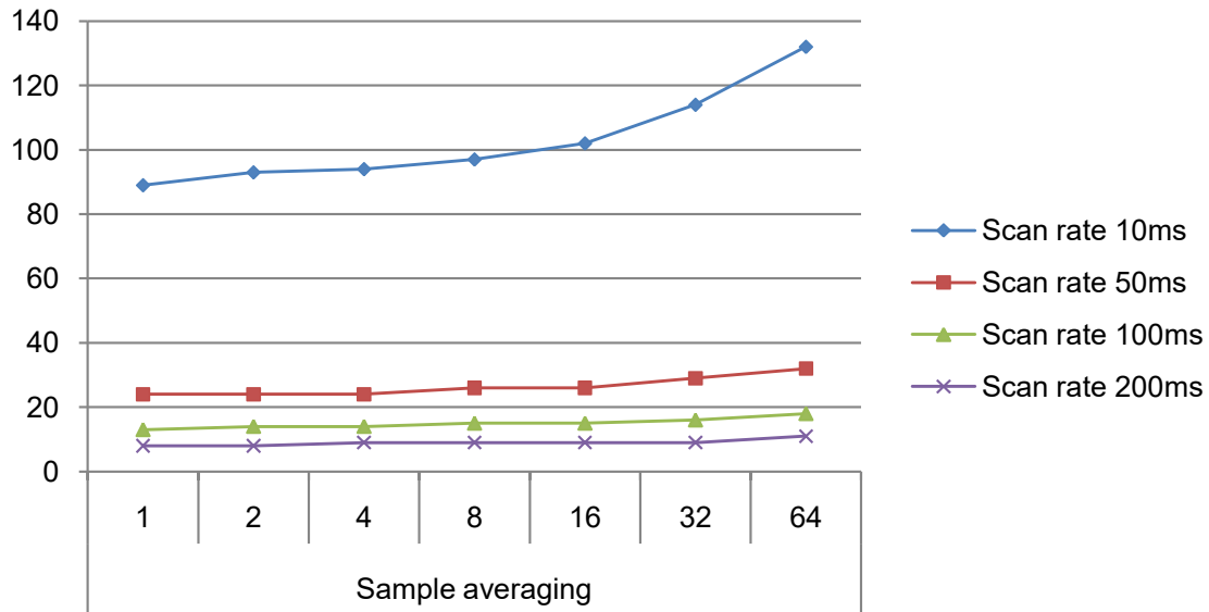
Figure 32-8. Power Consumption [ \mu A] 1 sensor, noise countermeasures Enabled, f=48\text{MHz} , V_{cc}=3.3\text{V}
