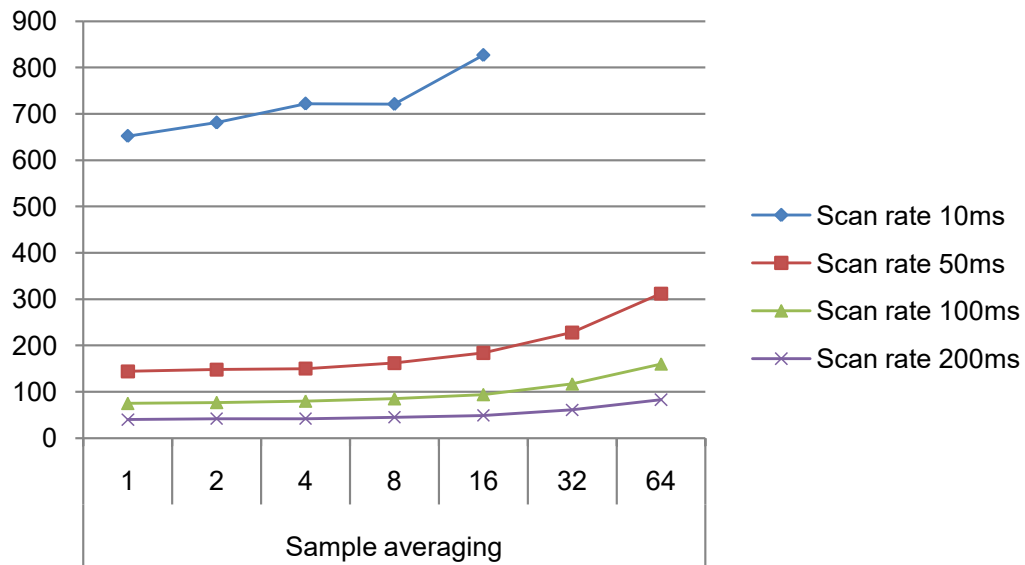
Figure 32-10. Power Consumption [ \mu A] 10 sensors, noise countermeasures Enabled, f=48\text{MHz} , V_{CC}=3.3\text{V}
