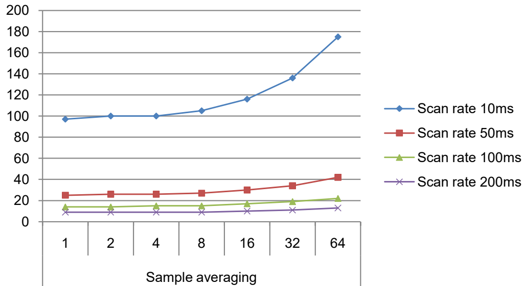
Figure 32-8. Power Consumption [ \mu A] 1 sensor, noise countermeasures Enabled, f=48\text{MHz} , V_{cc}=3.3\text{V}
