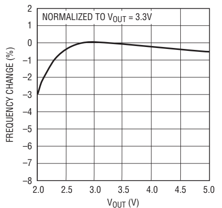
Oscillator Frequency vs V_{OUT}
