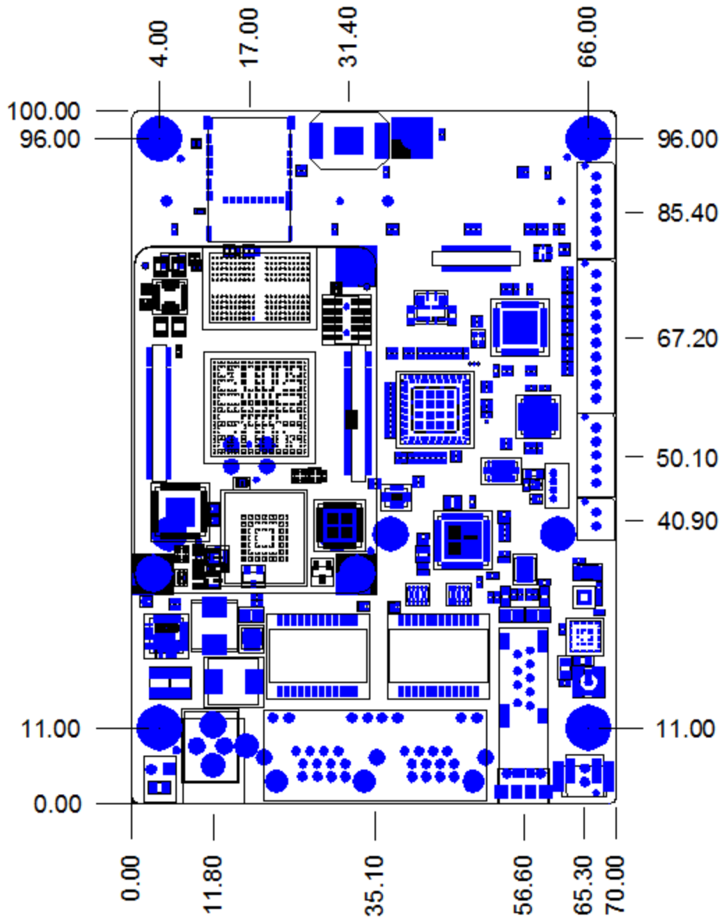
Top Side with Mechanical Dimensions
