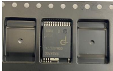
Existing Pocket Design
