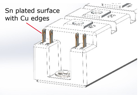
SEMITRANS 2 housing with auxiliary contacts
