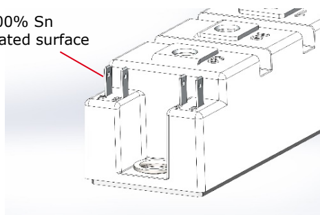
SEMITRANS 2 housing with auxiliary contacts
