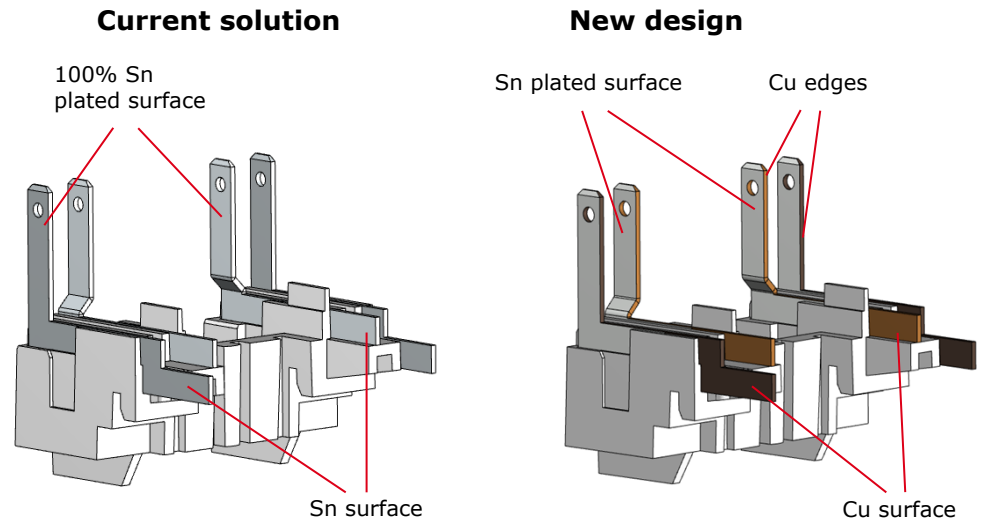
Auxiliary contacts with fixing base inside the housing
