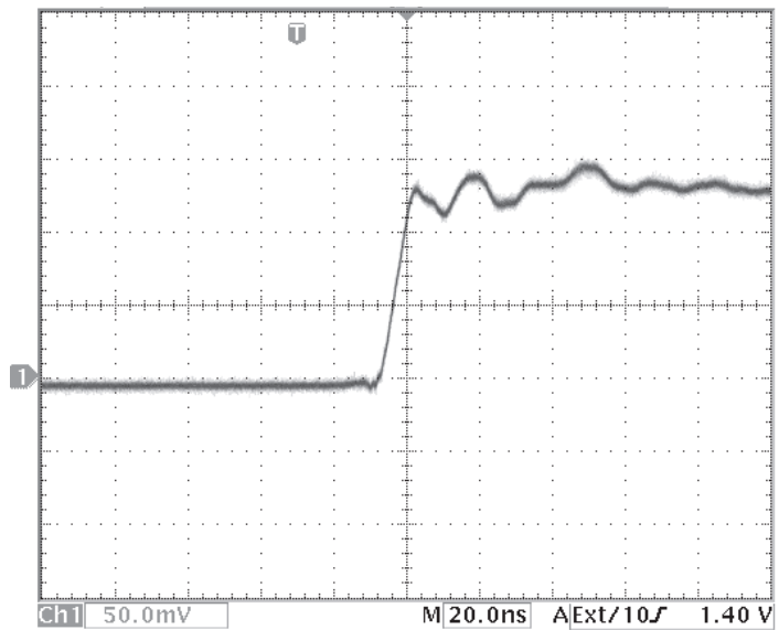
Figure 6 Rise Time 200x attenuation, 10%-90%
