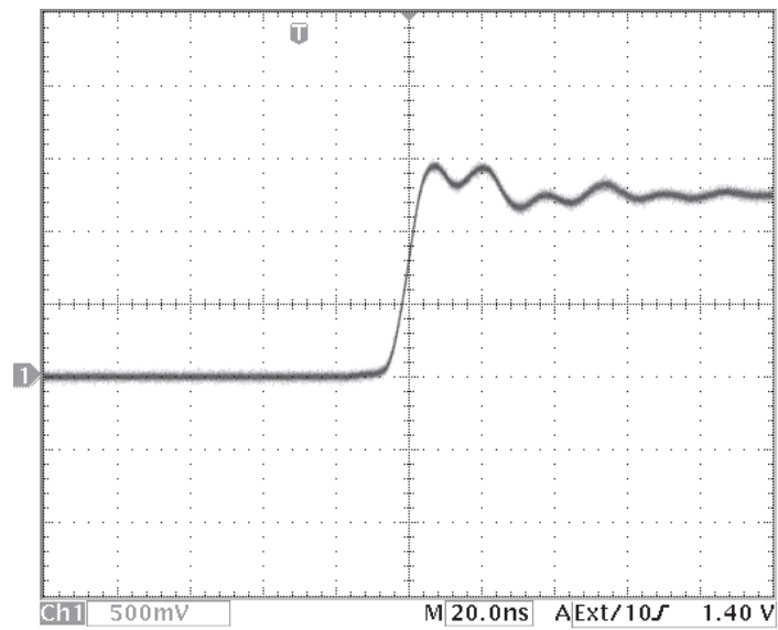
Figure 5 Rise Time 20x attenuation, 10%-90%
