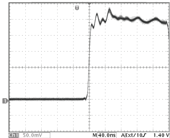
Figure 4 Rise Time
