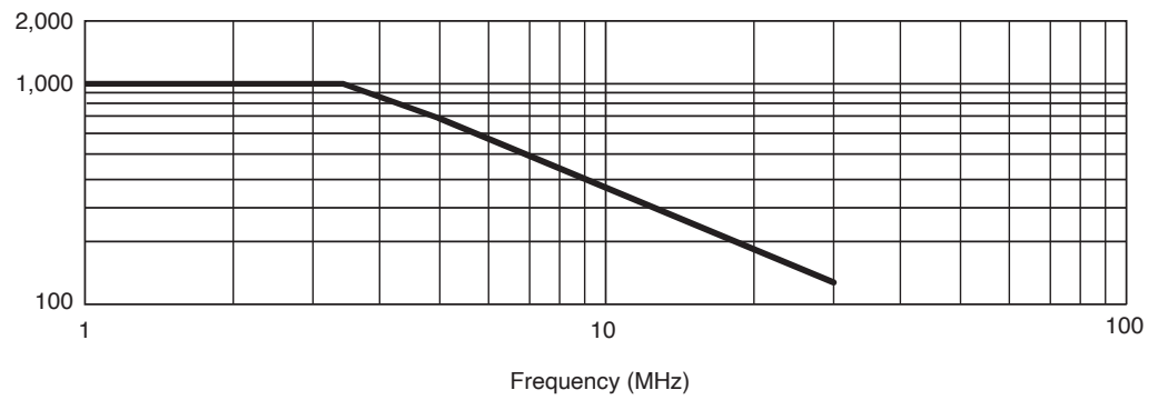
Figure 12 Typical Voltage Derating
