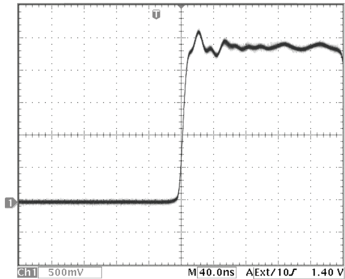
Figure 3 Rise Time
