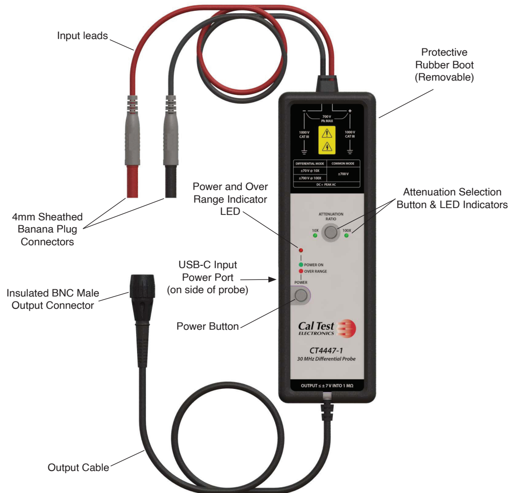
Figure 1 Probe and Supplied Accessories
