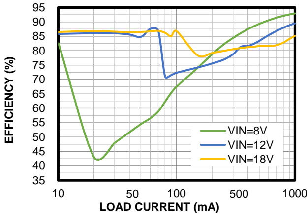
Efficiency vs. Load Current FCCM
