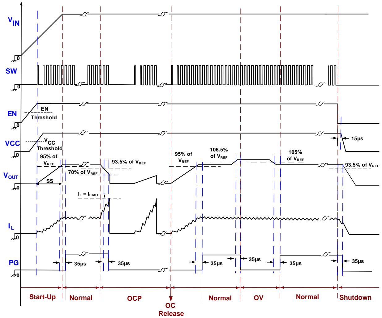
Figure 2: Timing Sequence
