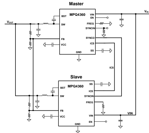
Figure 6: Dual-Phase Configuration
