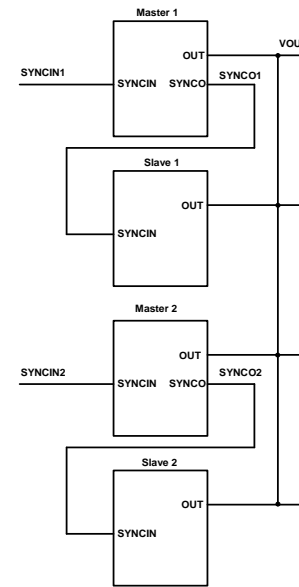
Figure 7: Four-Phase Configuration
