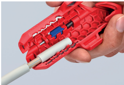
Dismantling of a NYM cable
