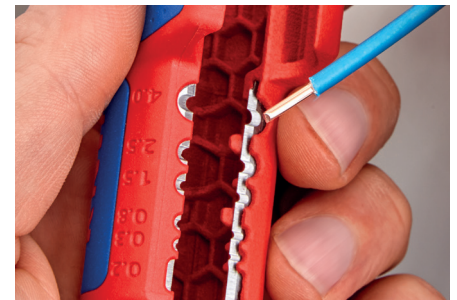
Stripping of single conductors
