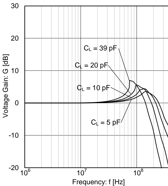
Figure 47. Voltage Gain vs Frequency (G = 0 dB, V_S = 2.7\text{ V} , R_L = 100\ \Omega )
