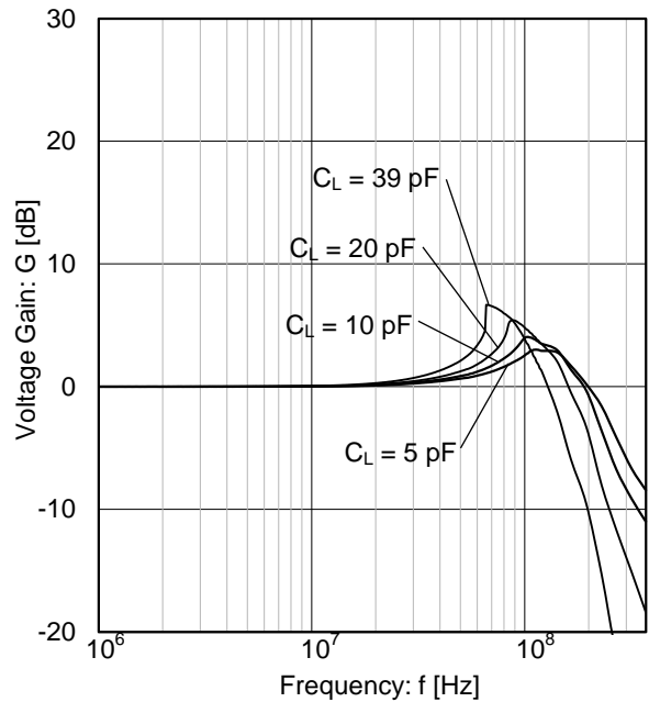
Figure 48. Voltage Gain vs Frequency (G = 0 dB, V_S = 5.5\text{ V} , R_L = 100\ \Omega )
