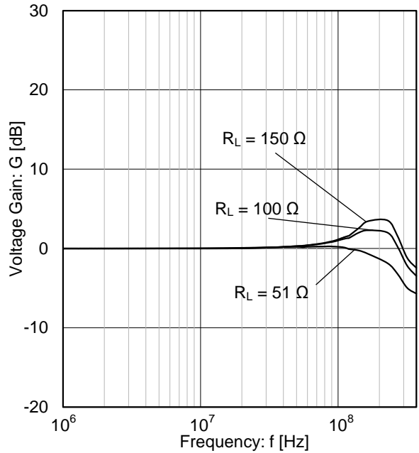
Figure 46. Voltage Gain vs Frequency (G = 0 dB, V_S = 5.5\text{ V} )
