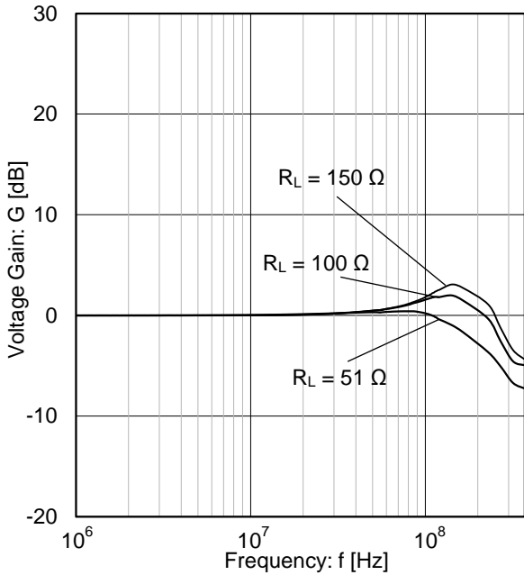
Figure 45. Voltage Gain vs Frequency (G = 0 dB, V_S = 2.7\text{ V} )
