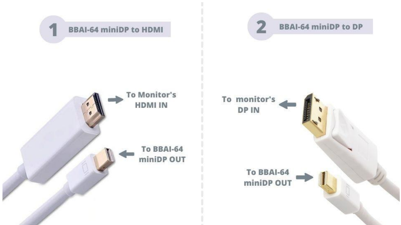
Figure 9. Connect miniDP-DP or active miniDP-HDMI cable to BeagleBone AI-64
