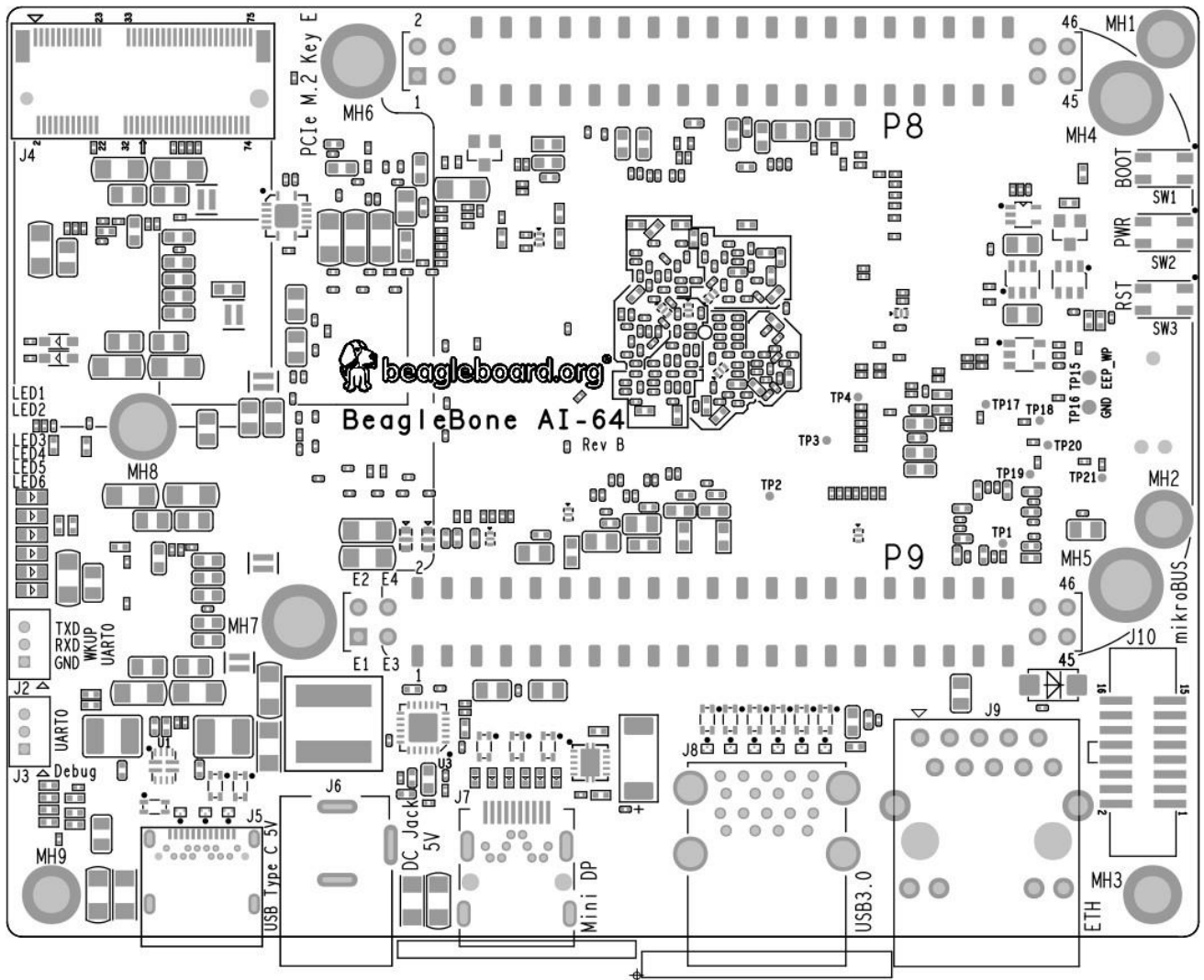
Figure 22. Bottom silkscreen
