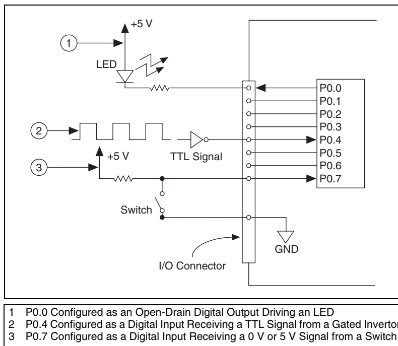
Figure 3-4. Example of Connecting a Load
